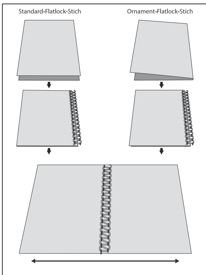
2-Faden-Flatlock-Stich
