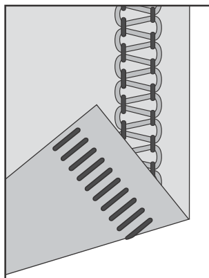
2-Faden-Flatlock-Stich
